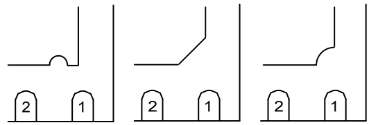
Pin 1 options
