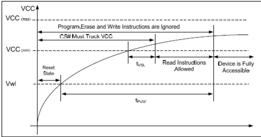
Figure 25 Power-up Timing
