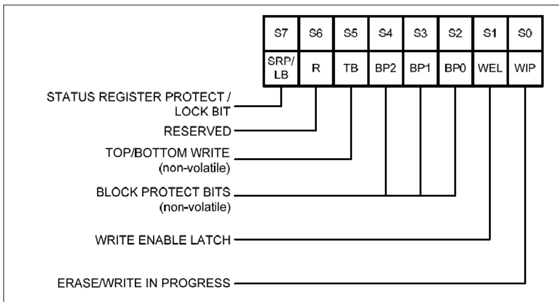
Figure 4 Status Register
