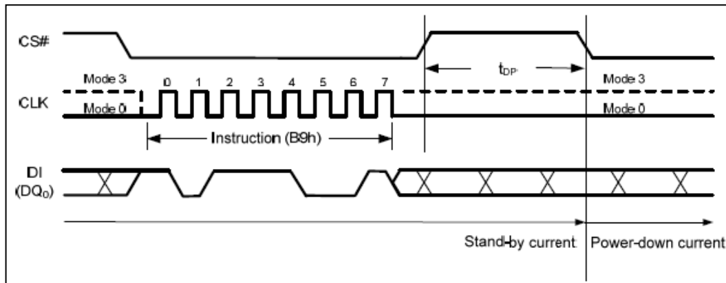
Figure 19 Deep power-down instruction
