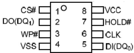
SOP-8
