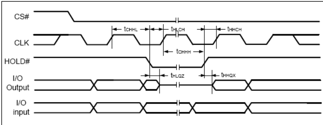
Figure 29 Hold timing
