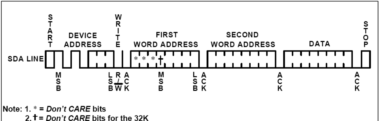
Figure 8. Byte Write
