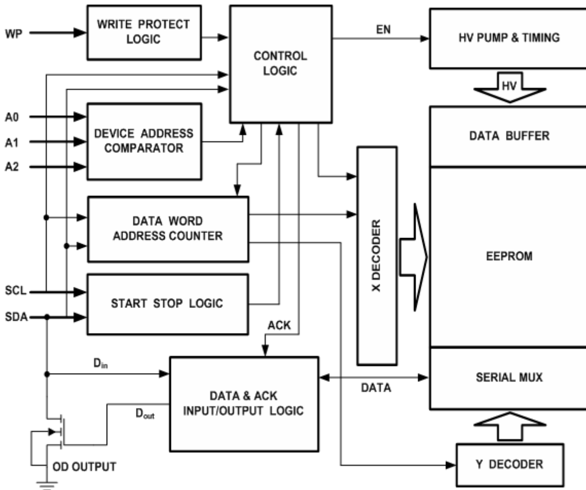
Figure 1. Block Diagram
