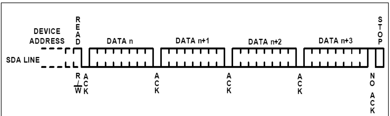
Figure 12. Sequential Read
