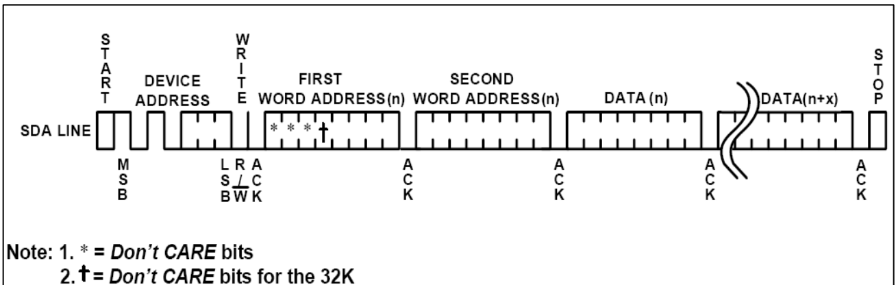
Figure 9. Page Write
