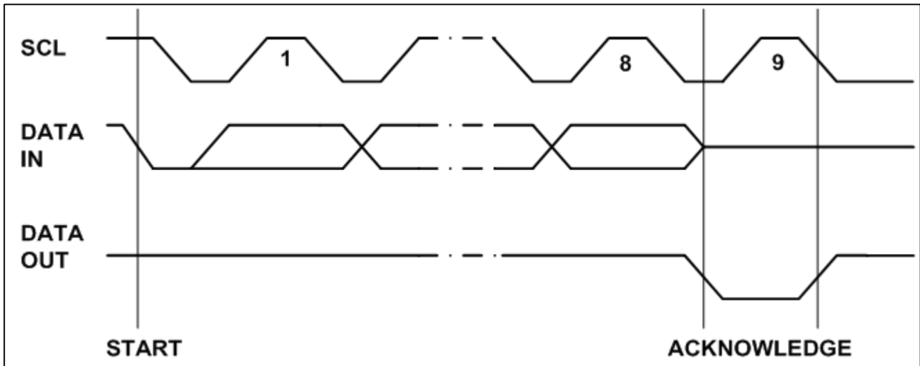
Figure 6. Output Acknowledge
