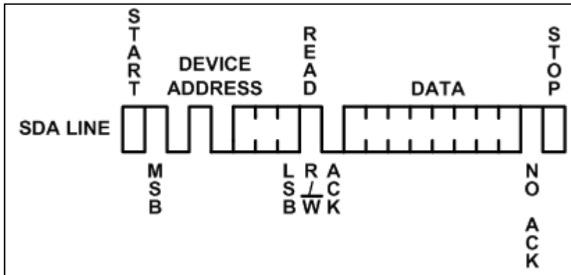
Figure 10. Current Address Read
