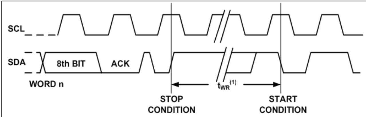
Figure 3. SCL: Serial Clock, SDA: Serial Data I/O
